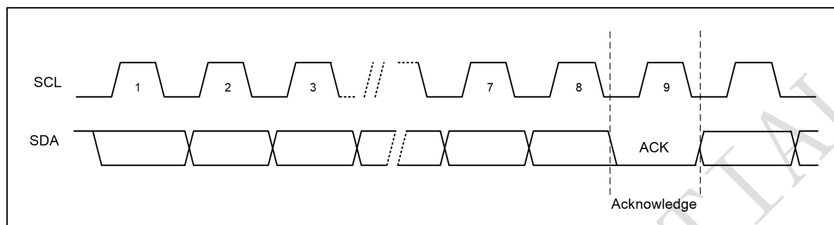
Figure 4-3 Output Acknowledge
