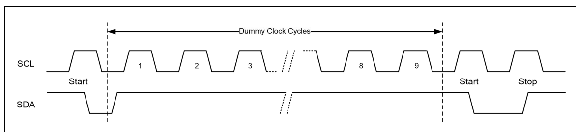
Figure 4-4 Soft Reset
