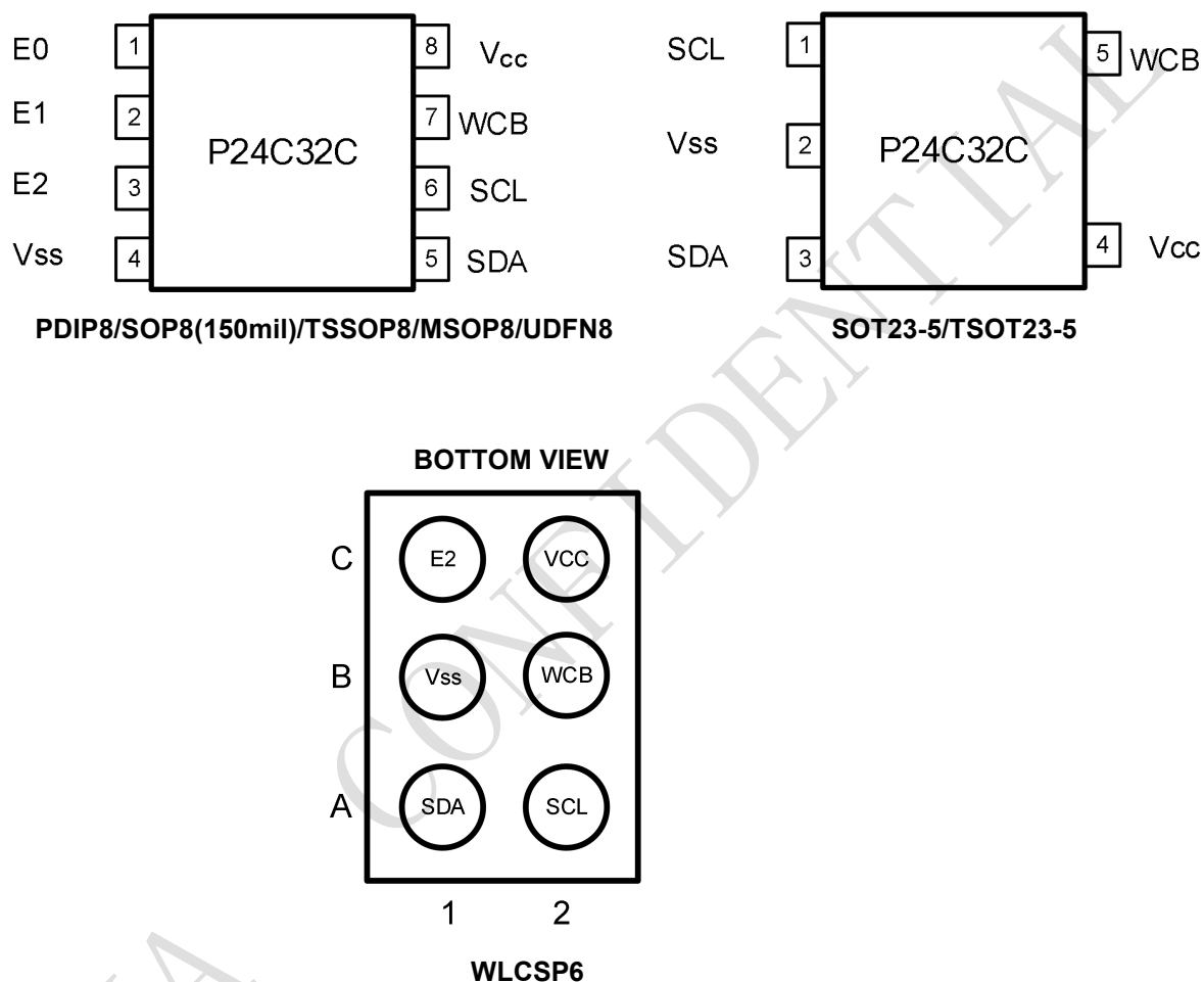
Figure 1-1 Pin Configuration
