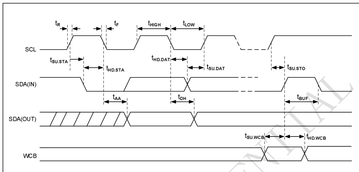
Figure 3-1 Bus Timing
